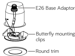
4" Recessed Housing
