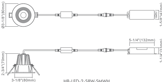
HB-LED-2-S8W-SMWH
