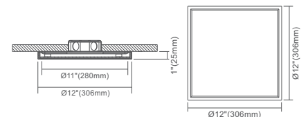
12" Die-cast Aluminum Square
