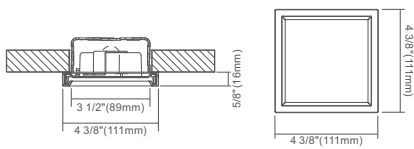
4" Plastic Square
