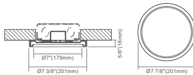
7" Plastic Round
