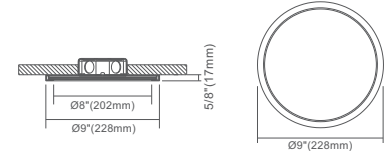
9" Plastic Round
