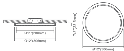
12" Plastic Round
