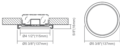
5" Plastic Round
