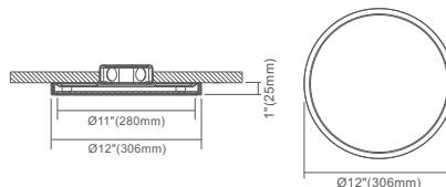
12" Die-cast Aluminum Round
