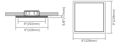
9" Plastic Square
