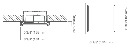
6" Plastic Square
